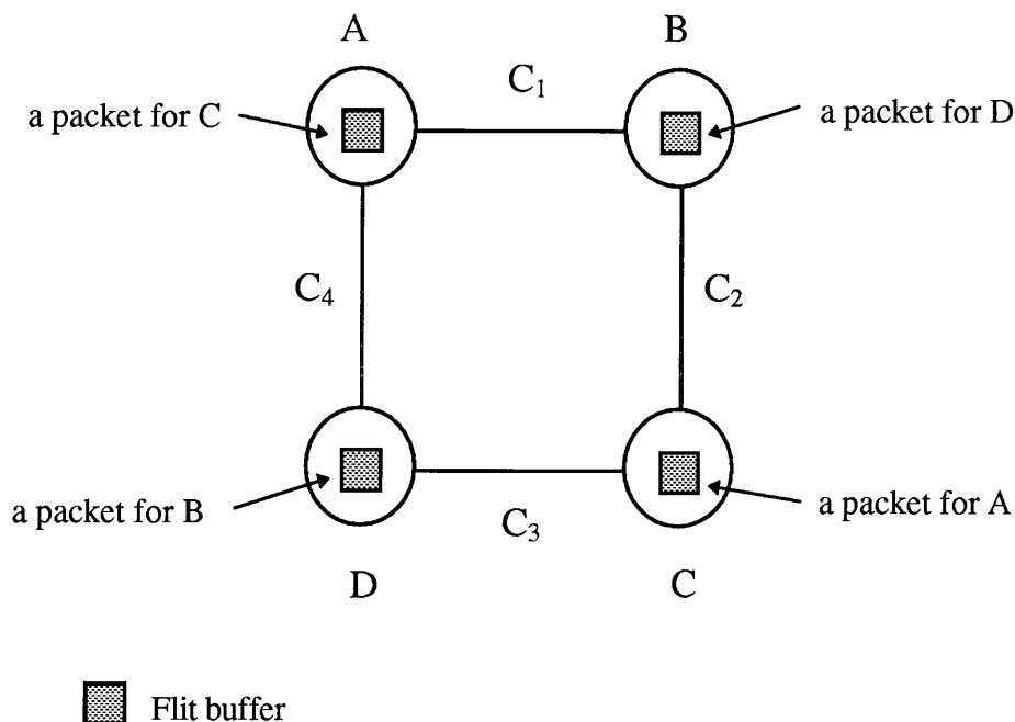
Figure 1.11: A deadlock in wormhole routing.
