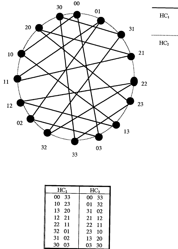
Figure 7.1: The 2 link-disjoint Hamiltonian cycles in a Q_2^4 .
