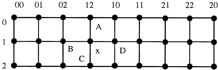
Figure 2.2: Embedding a 3^2 \times 3 mesh into a Q_3^3 .
