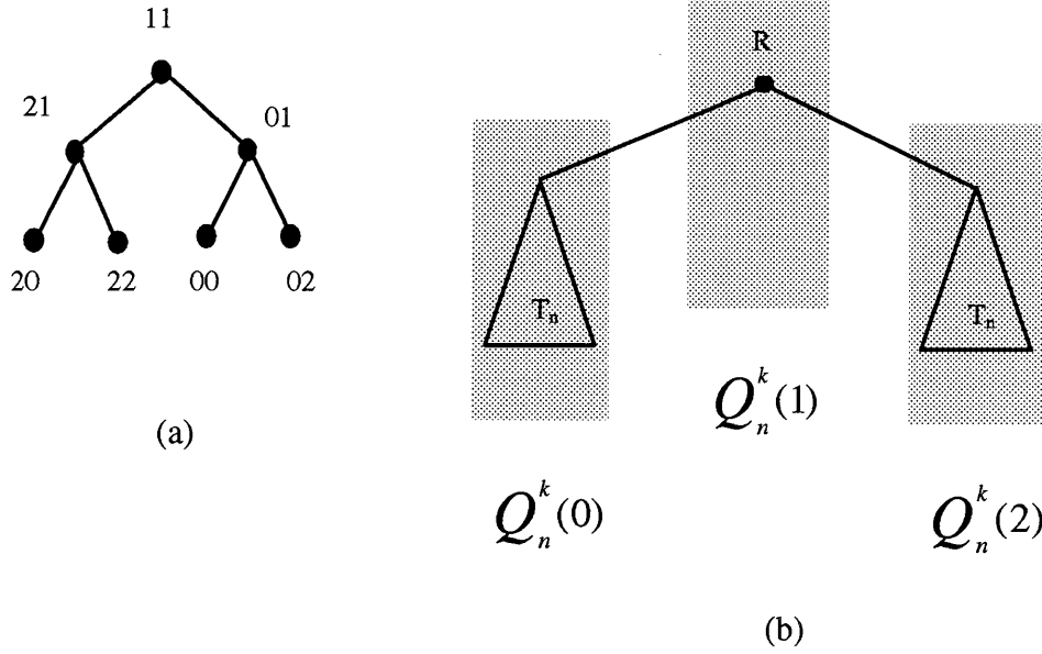
Figure 2.3: Embedding a complete binary tree T_n into a Q_n^k :
