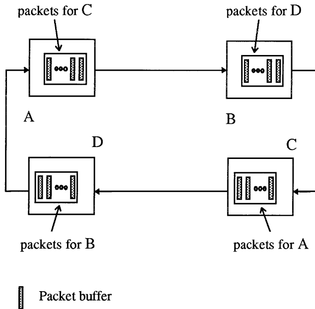
Figure 1.10: A deadlock in store-and-forward routing.
