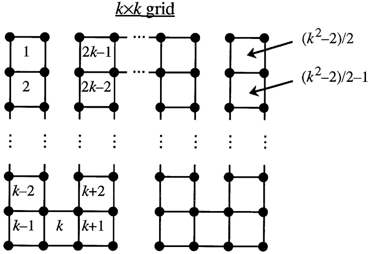
Figure 3.4: The tiled grid of Lemma 3.7.
